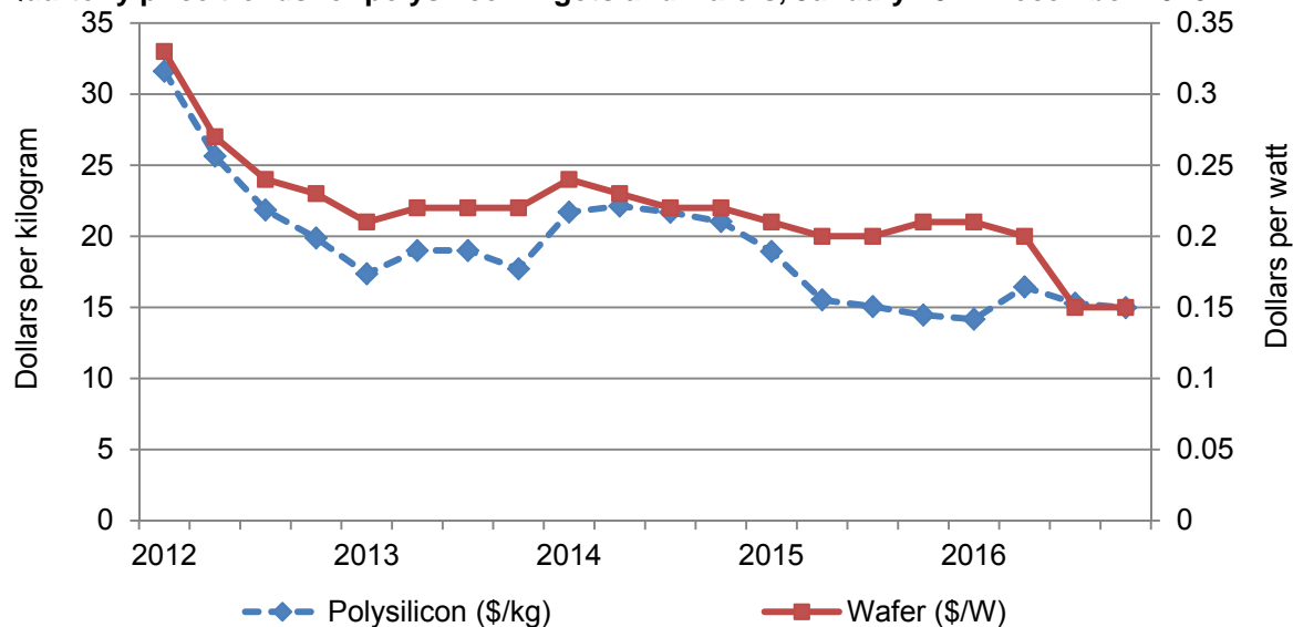
Figure V-7 Quarterly price trends for polysilicon ingots and wafers, January 2012-December 2016
