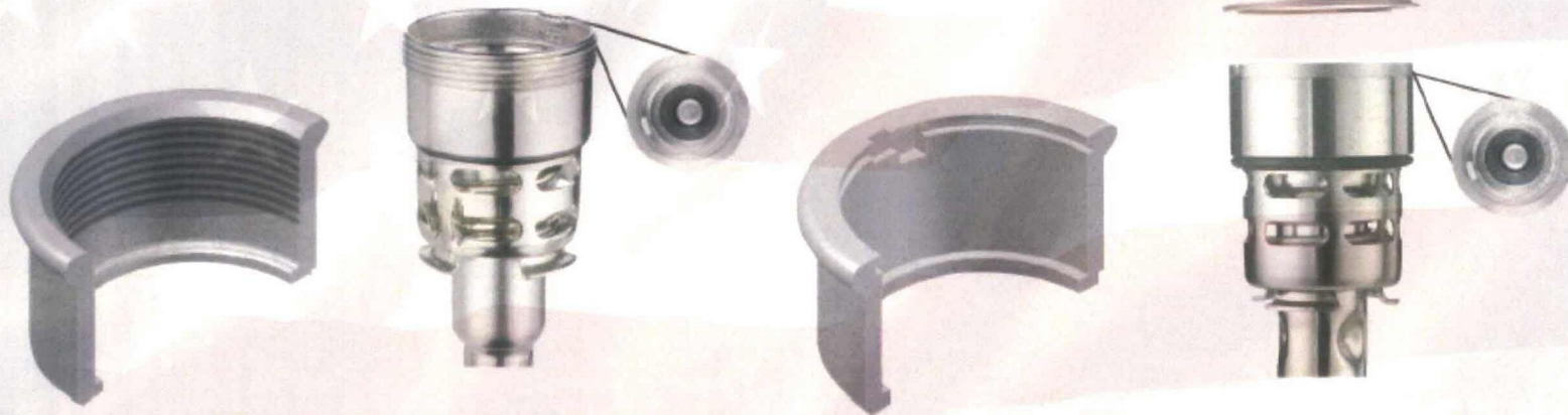
D-System Drop-In Valve with Retaining Ring
